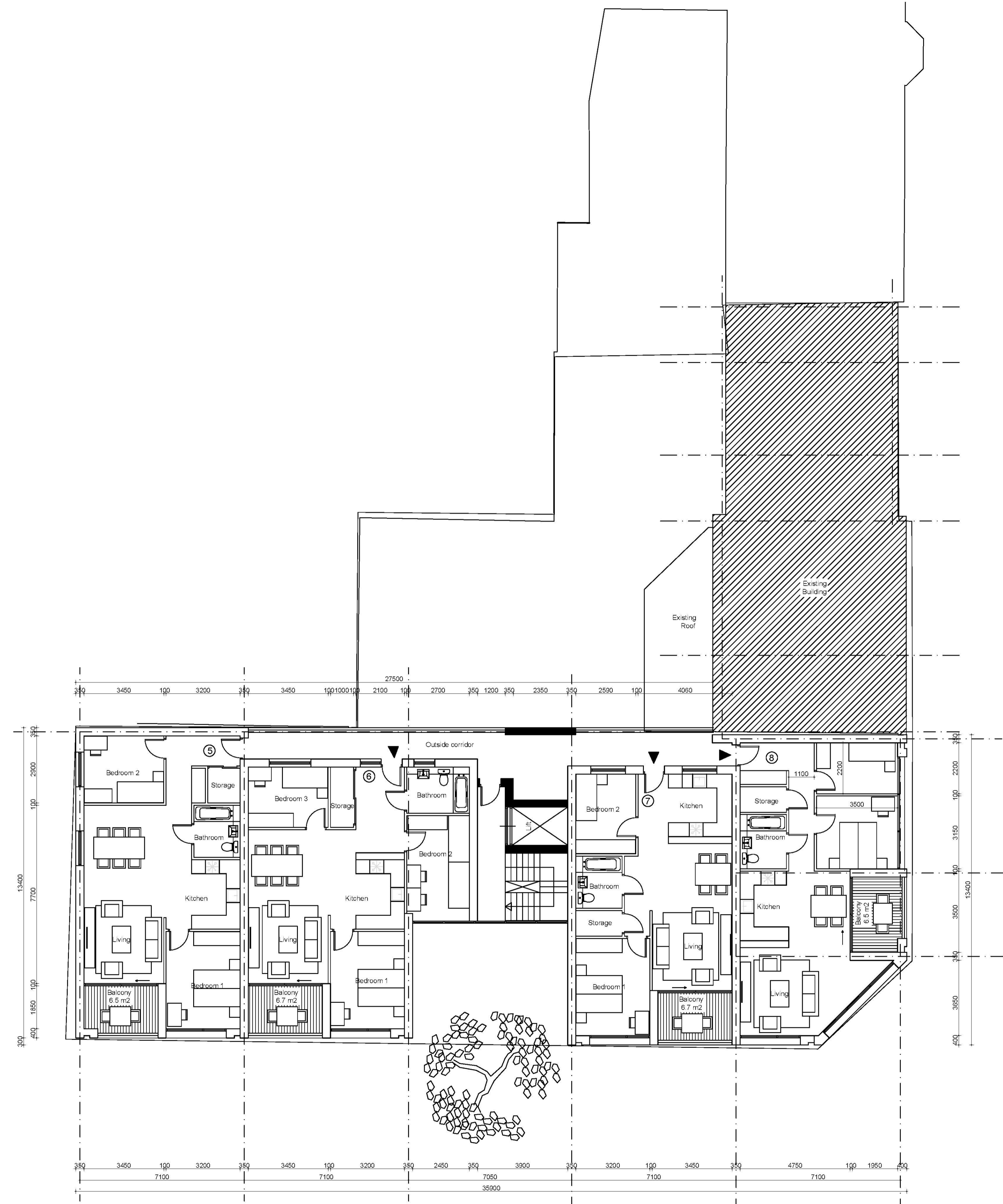
Proposed 2nd Floor Plan
